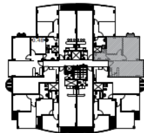
Typical Floor
